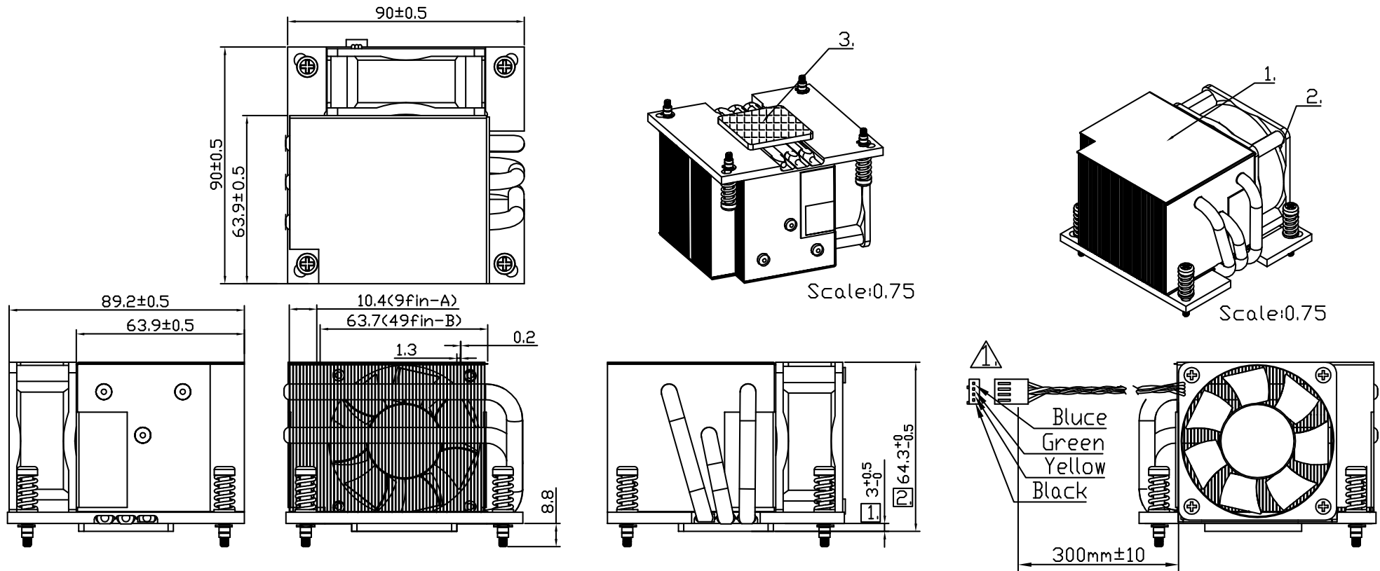
Figure 6 Cooler 125W mechanical dimension
