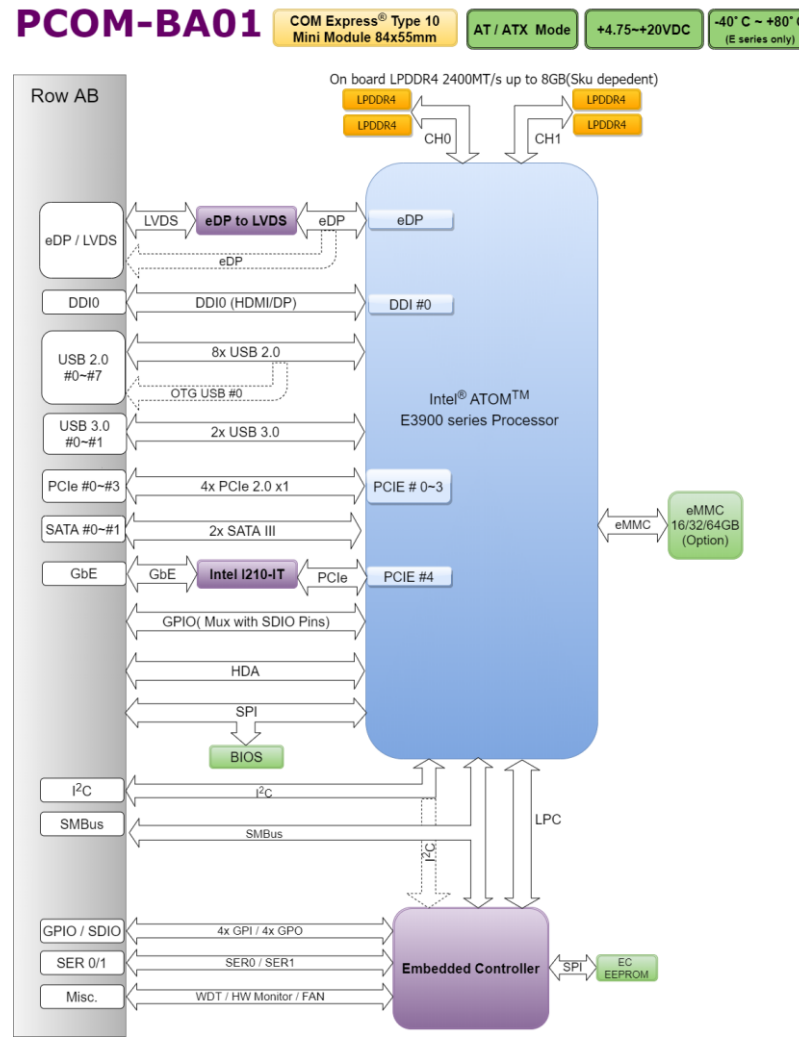
Figure 1 Block Diagram
