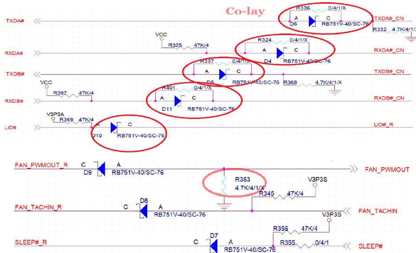
Figure 4 Circuit protection design
