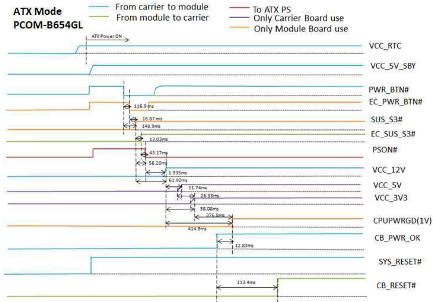
Figure 2 Power sequence ATX Mode
