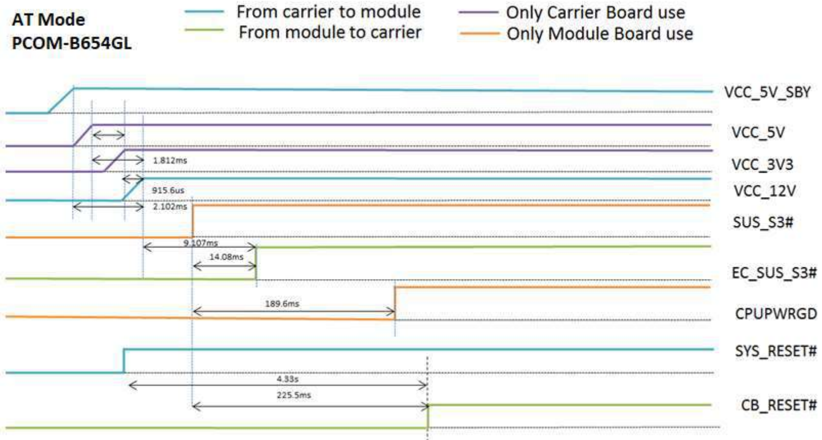
Figure 3 Power Sequence AT Mode
