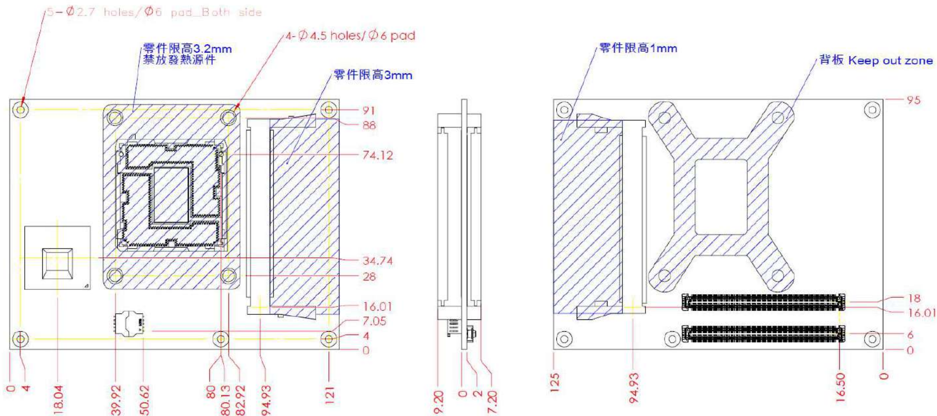
Figure 5 Mechanical Dimensions - Top/Bottom
