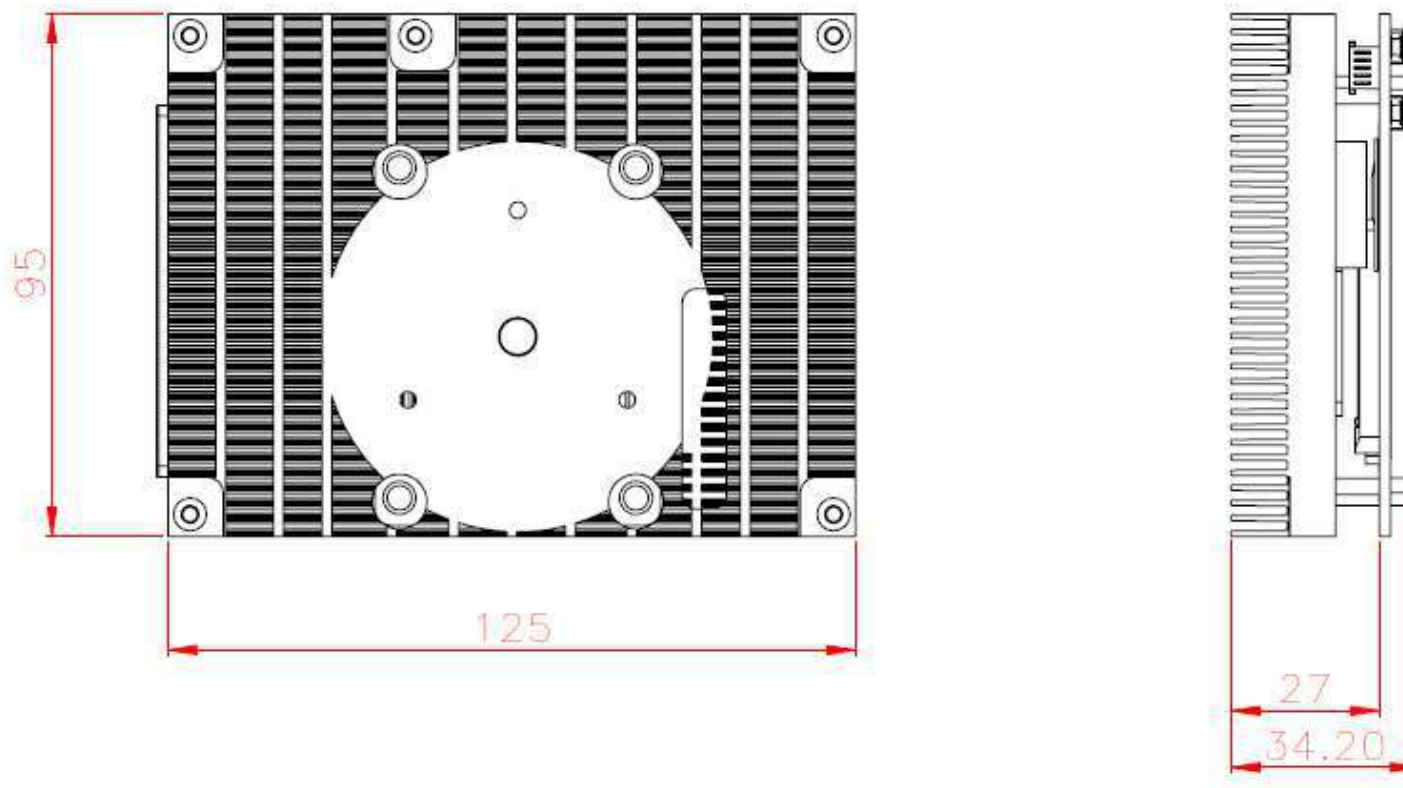
Figure 6 PCOM-B654GL with HS
