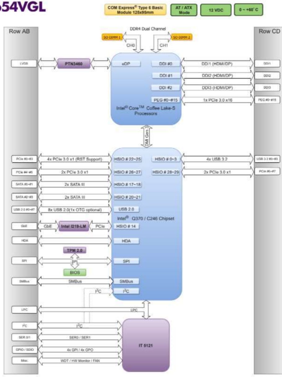
Figure 1 Block Diagram
