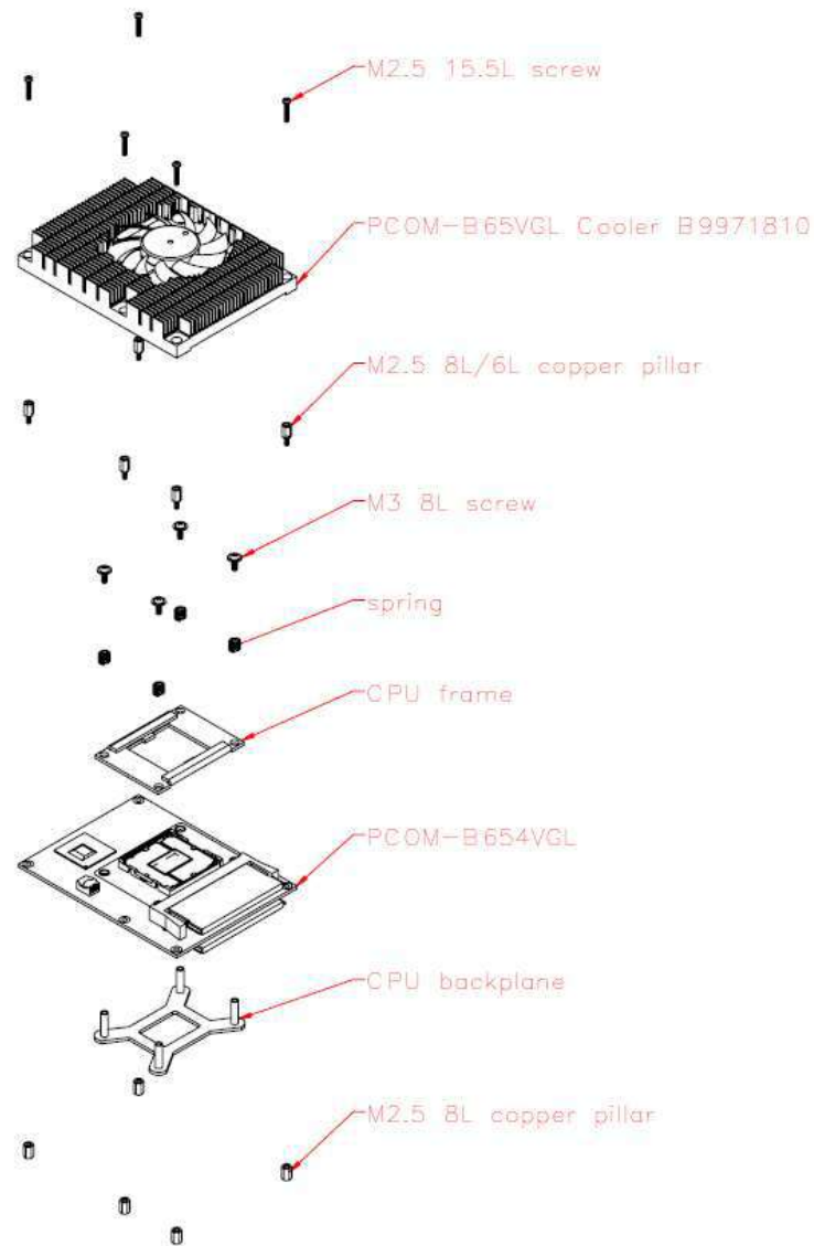
Figure 6 H/S Assembly guide
